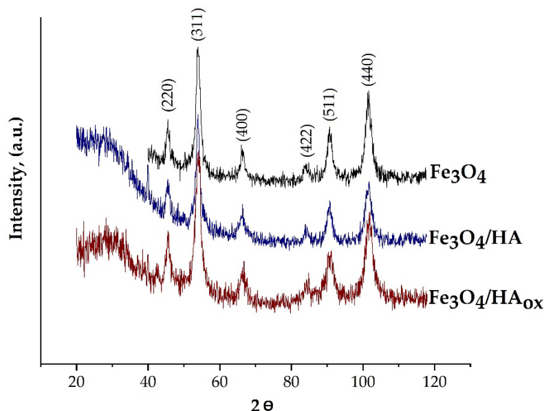
Fig. 1. XRD patterns of synthesized \text{Fe}_3\text{O}_4 nanoparticles. HA-humic acids. [6]
